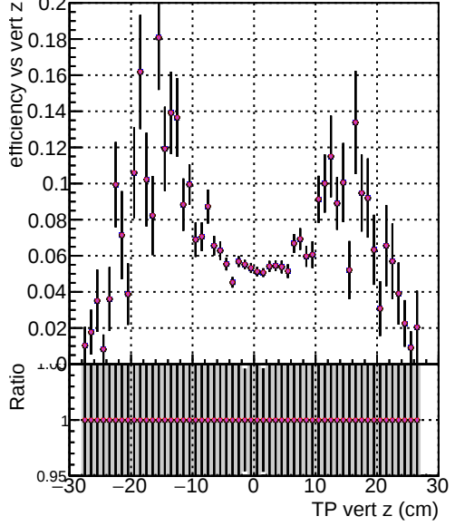
Efficiency vs. TP vert z DOM mkFit TT new-lowpt DOM mkFit TT NEWdefault specPLess1-lowpt DOM mkFit TT NEWdefault specPLess2-lowpt DOM mkFit TT NEWdefault specPLess3-lowpt DOM mkFit TT NEWdefault specPLess4-lowpt
