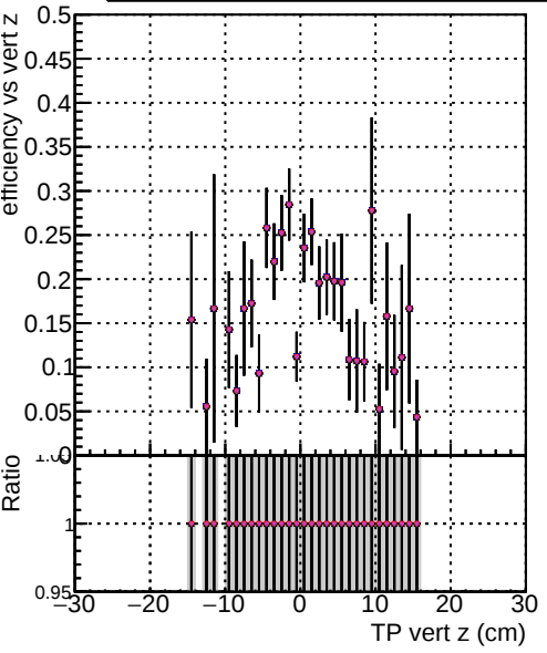
Efficiency vs vertpos DOM mkFit TT NEWdefault specPless1-lowpt DOM mkFit TT NEWdefault specPless2-lowpt DOM mkFit TT NEWdefault specPless3-lowpt DOM mkFit TT NEWdefault specPless4-lowpt
