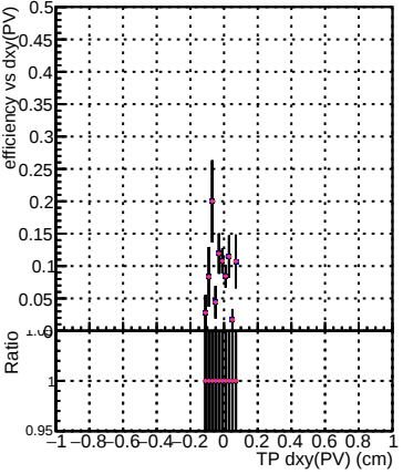
Efficiency vs Dxy(PV) DOM_mkFit_TT_NEWdefault_specPless1-lowpt DOM_mkFit_TT_NEWdefault_specPless2-lowpt DOM_mkFit_TT_NEWdefault_specPless3-lowpt DOM_mkFit_TT_NEWdefault_specPless4-lowpt
