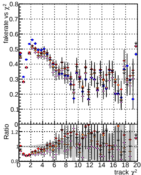
Fake rate vs. DDM mkt fit6 TTnew lowpt ttnew
