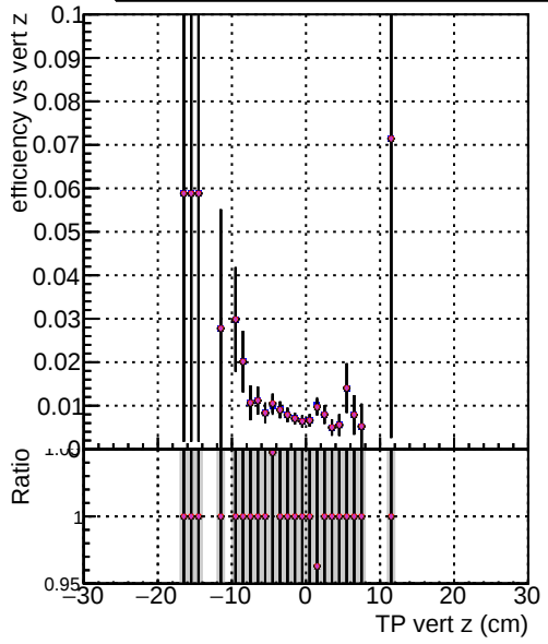
Efficiency vs vert z DOM mkFit XiMinusPU return DOM mkFit XiMinusPU NEWdefault specPLess1 DOM mkFit XiMinusPU NEWdefault specPLess2 DOM mkFit XiMinusPU NEWdefault specPLess3 DOM mkFit XiMinusPU NEWdefault specPLess4
