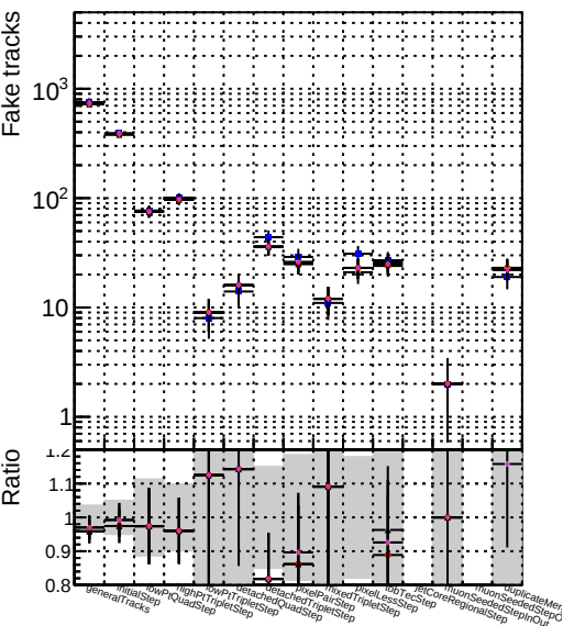
DOM mkFit XiMinusPU retrain DOM mkFit XiMinusPU NEWdefault specPless1 DOM mkFit XiMinusPU NEWdefault specPless2 DOM mkFit XiMinusPU NEWdefault specPless3 DOM mkFit XiMinusPU NEWdefault specPless4
