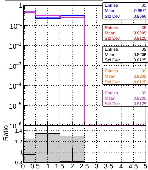
Legend: DOM mkFit XiMinusPU NEWdefault specPLess1 (blue), DOM mkFit XiMinusPU NEWdefault specPLess2 (red), DOM mkFit XiMinusPU NEWdefault specPLess3 (orange), DOM mkFit XiMinusPU NEWdefault specPLess4 (purple) mean hit
