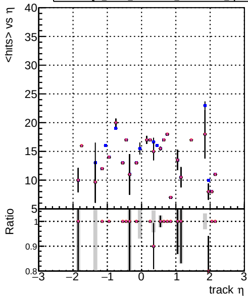
Legend: DOM mkFit XiMinusPU NEWdefault specPLess1 (blue), DOM mkFit XiMinusPU NEWdefault specPLess2 (red), DOM mkFit XiMinusPU NEWdefault specPLess3 (orange), DOM mkFit XiMinusPU NEWdefault specPLess4 (purple) mean hit
