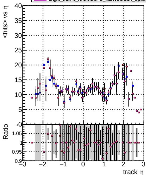
mean hits DOM mkFit XiMinusPU NEWdefault specPless1 DOM mkFit XiMinusPU NEWdefault specPless2 DOM mkFit XiMinusPU NEWdefault specPless3 DOM mkFit XiMinusPU NEWdefault specPless4
