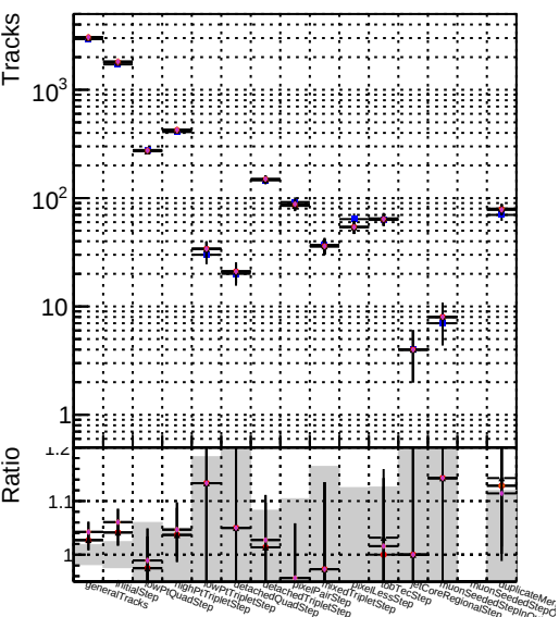
DOM mkFit XiMinusPU tetraim DOM mkFit XiMinusPU NEWdefault specPless1 DOM mkFit XiMinusPU NEWdefault specPless2 DOM mkFit XiMinusPU NEWdefault specPless3 DOM mkFit XiMinusPU NEWdefault specPless4
