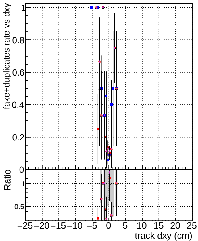
DOM_mkFit_XiMinusPU_retrain DOM_mkFit_XiMinusPU_NEWdefault_specPLess1 DOM_mkFit_XiMinusPU_NEWdefault_specPLess2 DOM_mkFit_XiMinusPU_NEWdefault_specPLess3 DOM_mkFit_XiMinusPU_NEWdefault_specPLess4
