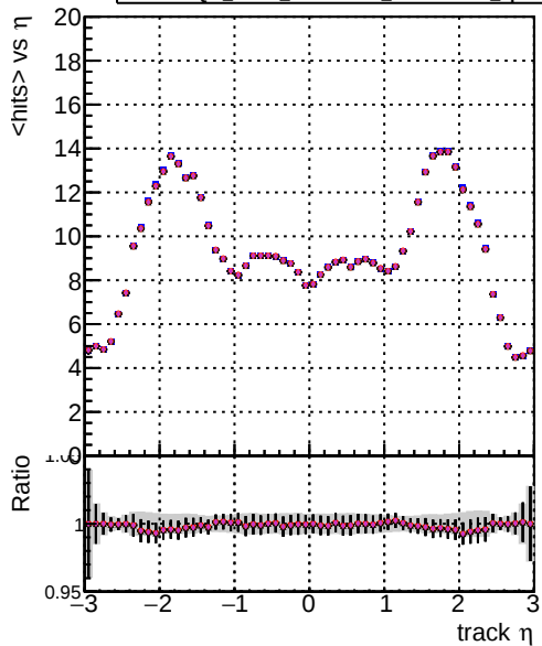
Legend for mean hits vs \eta : DOM mkFit XiMinusPU NEWdefault specPLess1 DOM mkFit XiMinusPU NEWdefault specPLess2 DOM mkFit XiMinusPU NEWdefault specPLess3 DOM mkFit XiMinusPU NEWdefault specPLess4
