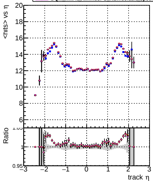
mean hits DOM mkFit XiMinusPU NEWdefault specPless1 DOM mkFit XiMinusPU NEWdefault specPless2 DOM mkFit XiMinusPU NEWdefault specPless3 DOM mkFit XiMinusPU NEWdefault specPless4
