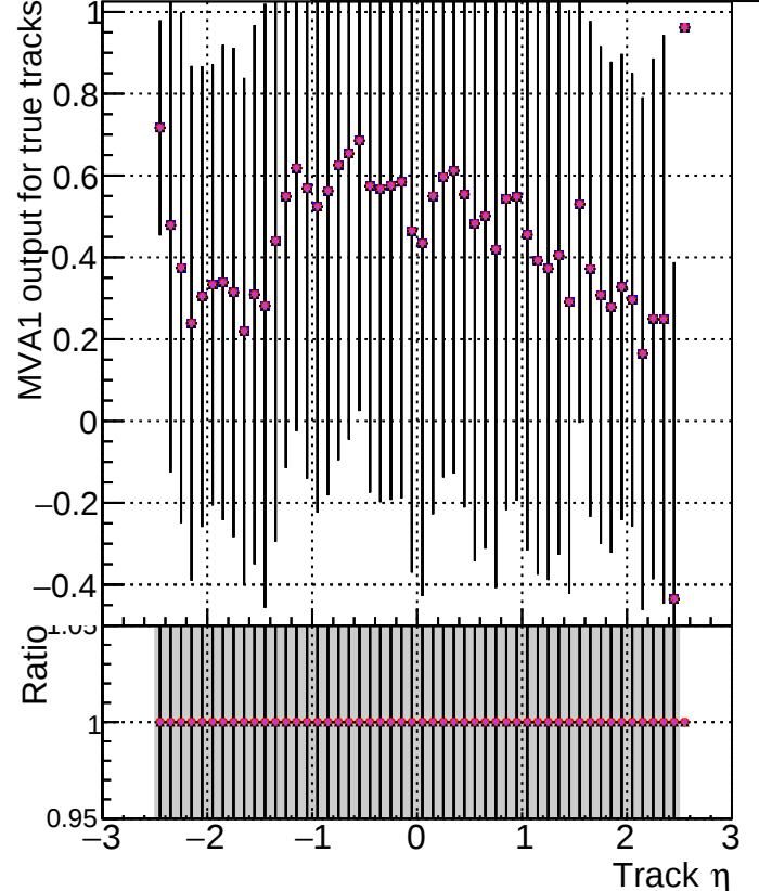
MVA1 of associated tracks (recoToSim) vs. track \eta Legend: DOM mkFit XiMinusPU retrain DOM mkFit XiMinusPU NEWdefault specPless1 DOM mkFit XiMinusPU NEWdefault specPless2 DOM mkFit XiMinusPU NEWdefault specPless3 DOM mkFit XiMinusPU NEWdefault specPless4
