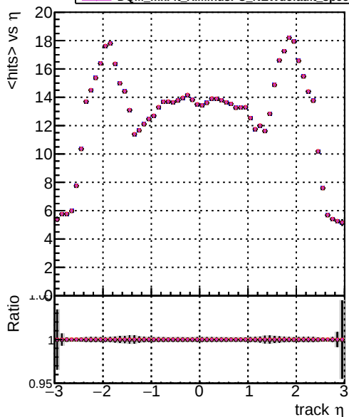
mean hit DOM mkFit XiMinusPU NEWdefault specPLess1 DOM mkFit XiMinusPU NEWdefault specPLess2 DOM mkFit XiMinusPU NEWdefault specPLess3 DOM mkFit XiMinusPU NEWdefault specPLess4
