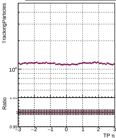
N of sim Legend DOM mkFit XiMinusPU NEWdefault specP Less2 Black line with star DOM mkFit XiMinusPU NEWdefault specP Less2 Red line with star DOM mkFit XiMinusPU NEWdefault specP Less3 Blue line with star DOM mkFit XiMinusPU NEWdefault specP Less4
