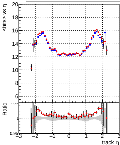
mean hits vs \eta Legend: DQM_mkFit_XiMinusPU_retrain2 (blue line), DQM_mkFit_XiMinusPUold (red line)
