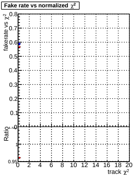
Fake rate vs. Legend: DQM_mkFit_XiMinusPU_retrain2 (blue) DQM_mkFit_XiMinusPUold (red)
