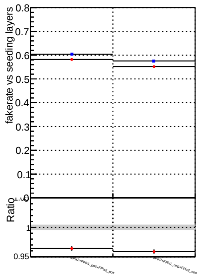
Fake rate vs. Legend: DQM_mkFit_XiMinusPU_retrain2 (blue) DQM_mkFit_XiMinusPUold (red)
