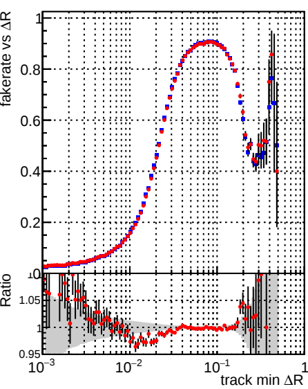
Fake rate vs \Delta R(\text{track, jet}) Legend: \blacksquare DQM_mkFit_XiMinusPU_retrain2 \bullet DQM_mkFit_XiMinusPUold
