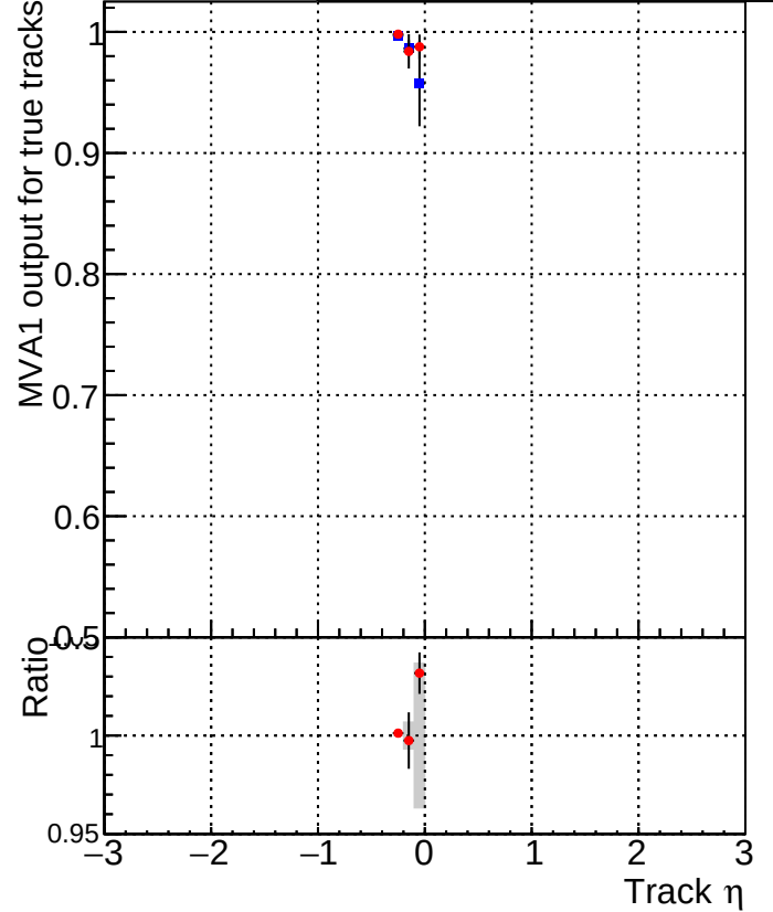
MVA1 of associated tracks (recoToSim) vs. track \eta Legend: ■ DQM_mkFit_XiMinusPU_retrain2 ● DQM_mkFit_XiMinusPUold
