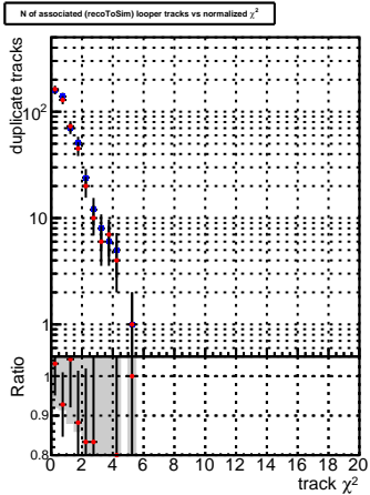
associated looper tracks vs. \chi^2
