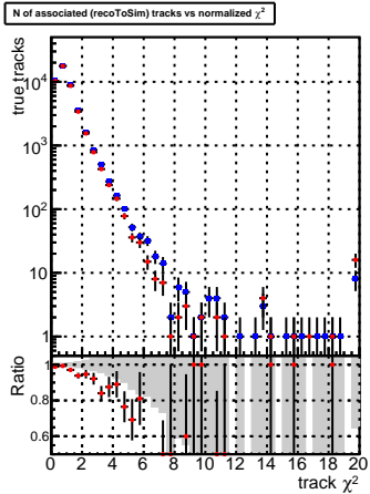
associated tracks vs. \chi^2
