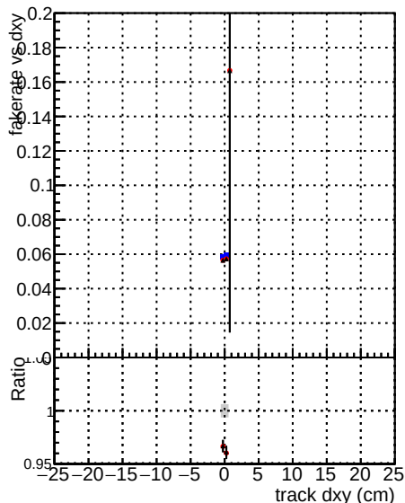
Fake rate vs d DOM mkFit5 XIMinusPUold DOM mkFit5 XIMinusPU retrain2 DOM mkFit5 XIMinusPU NEWdefault specPLess3-2
