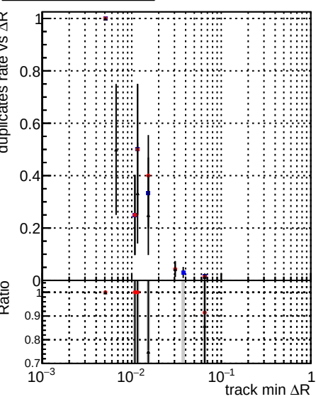
Legend: DQM_mkFit5_XiMinusPUold (blue squares), DQM_mkFit_XiMinusPU_retrain2 (red circles), DQM_mkFit_XiMinusPU_renewdefault_specPLess3-2 (black circles)
