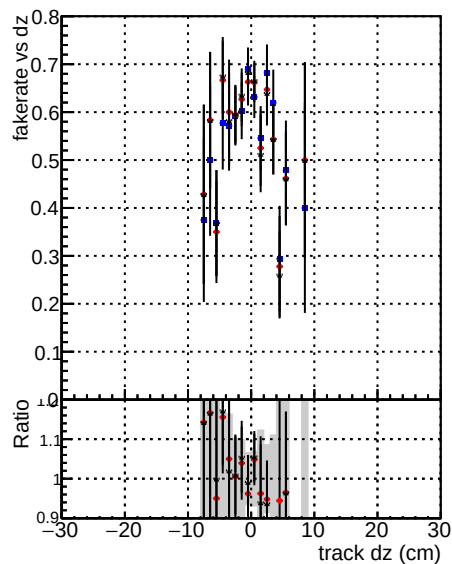
Fake rate vs dz Legend: DOM mkFit5 (black line) XiMinusPUold (blue line) XiMinusPU (red line) XiMinusPU Ntrain2 (grey line) NEWdefault (black line) specPLESS3-2 (black line)
