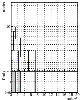
N of reco track vs. \chi^2 for various algorithms
