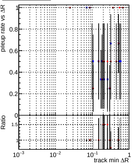
Legend: DQM_mkFit5_XiMinusPUold (blue dots), DQM_mkFit5_XiMinusPU_retrain2 (red dots), DQM_mkFit5_XiMinusPU_NEWdefault_specPLess3-2 (black dots)
