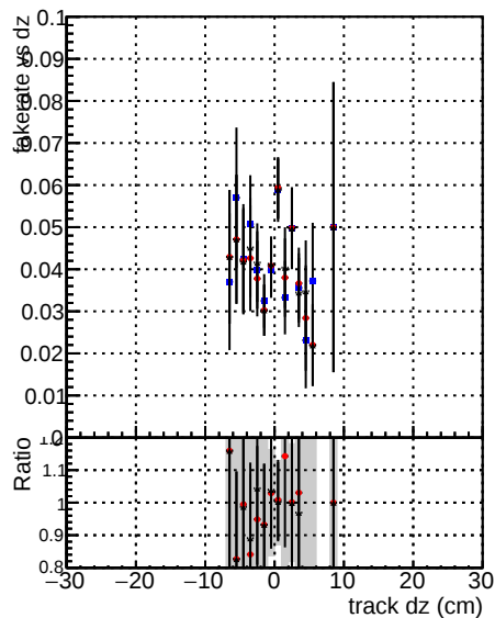
Fake rate vs d DOM mkFit5 XMinusPUold DOM mkFit XMinusPU retrain2 DOM mkFit XMinusPU NEWdefault specPLess3-2
