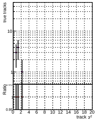
N of reco track vs. \chi^2 for different reconstruction methods
