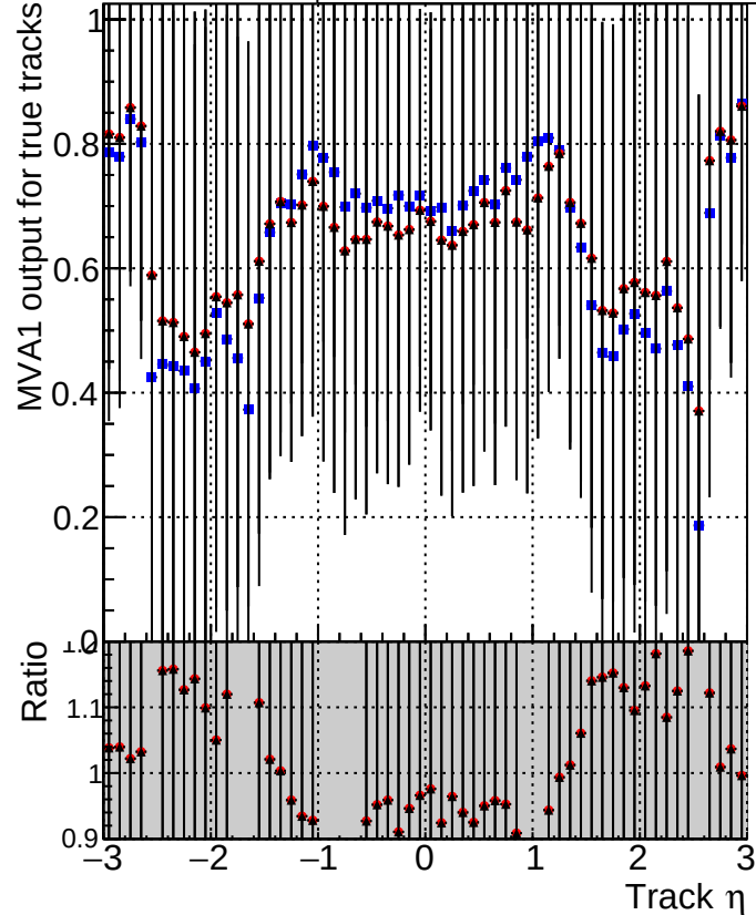
MVA1 of associated tracks (recoToSim) vs. track \eta ■ DQM_mkFit5_XiMinusPUold ● DQM_mkFit5_XiMinusPU_retrain2 ▲ DQM_mkFit5_XiMinusPU_NEWdefault_specPLess3-2
