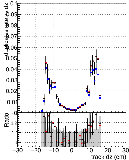
— DOM mkFit5 XiMinusPUold — DOM mkFit5 XiMinusPUnewtrain2 — DOM mkFit5 XiMinusPUnewdefault specPLESS3-2
