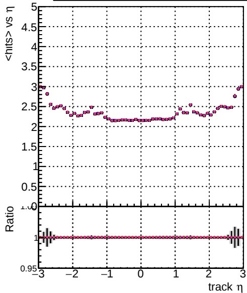
mean hit DOM mkFit XiMinusPU tetaIn-lowpt specPless1-lowpt DOM mkFit XiMinusPU NEWdefault specPless1-lowpt DOM mkFit XiMinusPU NEWdefault specPless3-lowpt DOM mkFit XiMinusPU NEWdefault specPless4-lowpt
