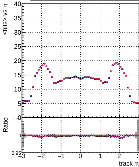
Legend for mean hits vs \eta : DOM mkFit XiMinusPU NEWdefault specPless1-lowpt DOM mkFit XiMinusPU NEWdefault specPless2-lowpt DOM mkFit XiMinusPU NEWdefault specPless3-lowpt DOM mkFit XiMinusPU NEWdefault specPless4-lowpt
