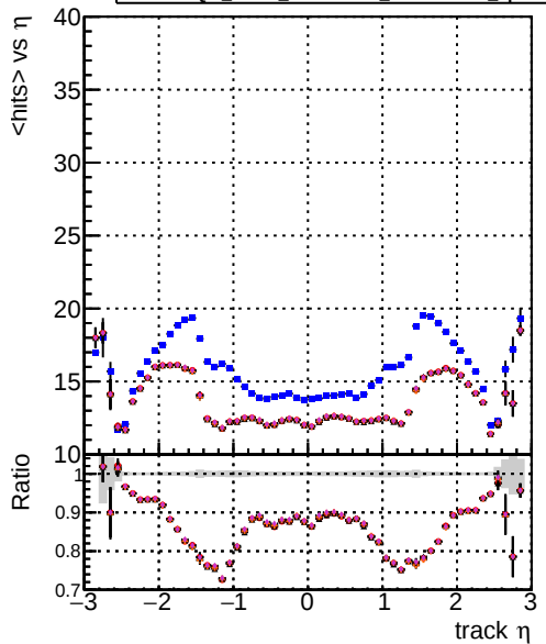
mean hits vs \eta DOM mkFit XiMinusPU tetaair-lowpt specPless1-lowpt DOM mkFit XiMinusPU NEWdefault specPless2-lowpt DOM mkFit XiMinusPU NEWdefault specPless3-lowpt DOM mkFit XiMinusPU NEWdefault specPless4-lowpt
