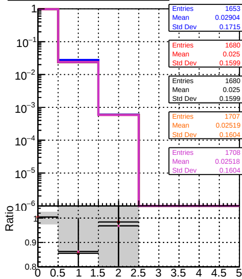
Legend for mean hits vs \eta : DOM mkFit XiMinusPU tetaIn-lowpt DOM mkFit XiMinusPU NEWdefault specPless1-lowpt DOM mkFit XiMinusPU NEWdefault specPless2-lowpt DOM mkFit XiMinusPU NEWdefault specPless3-lowpt DOM mkFit XiMinusPU NEWdefault specPless4-lowpt
