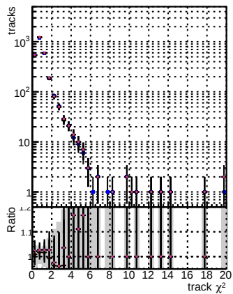
N of reco track vs. \chi^2 for different algorithms
