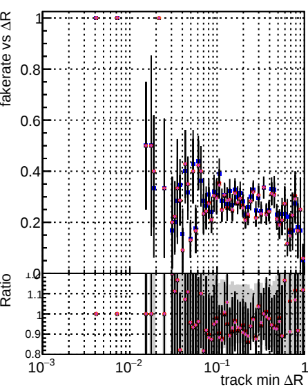
Fake rate vs \Delta R(\text{track, jet}) DQM mkFit XMinusPU retrain_lowpt specBLess1-lowpt specBLess2-lowpt specBLess3-lowpt specBLess4-lowpt
