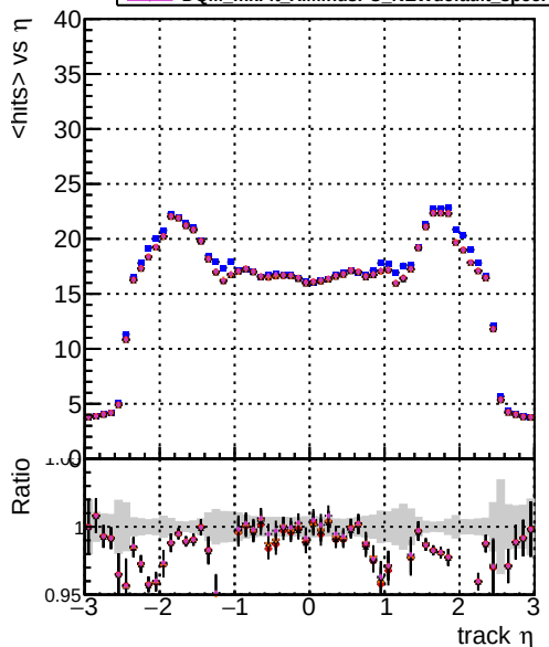
mean hit DOM mkFit XiMinusPU NEWdefault specPless1-lowpt DOM mkFit XiMinusPU NEWdefault specPless2-lowpt DOM mkFit XiMinusPU NEWdefault specPless3-lowpt DOM mkFit XiMinusPU NEWdefault specPless4-lowpt
