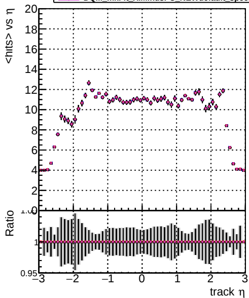
mean hits DOM mkFit XiMinusPU tetaInLowpt specPless1-lowpt DOM mkFit XiMinusPU NEWdefault specPless2-lowpt DOM mkFit XiMinusPU NEWdefault specPless3-lowpt DOM mkFit XiMinusPU NEWdefault specPless4-lowpt
