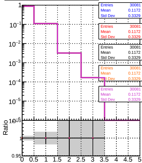
mean hits DOM mkFit XiMinusPU tetaInLowpt specPless1-lowpt DOM mkFit XiMinusPU NEWdefault specPless2-lowpt DOM mkFit XiMinusPU NEWdefault specPless3-lowpt DOM mkFit XiMinusPU NEWdefault specPless4-lowpt
