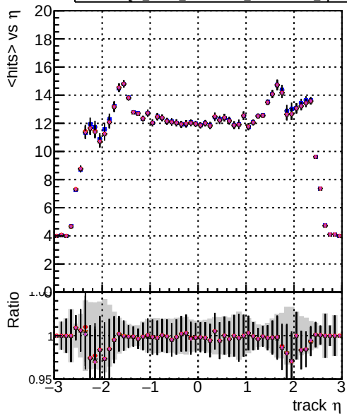
mean hit DOM mkFit XiMinusPU tetrailowpt specPless1-lowpt DOM mkFit XiMinusPU NEWdefault specPless1-lowpt DOM mkFit XiMinusPU NEWdefault specPless3-lowpt DOM mkFit XiMinusPU NEWdefault specPless4-lowpt
