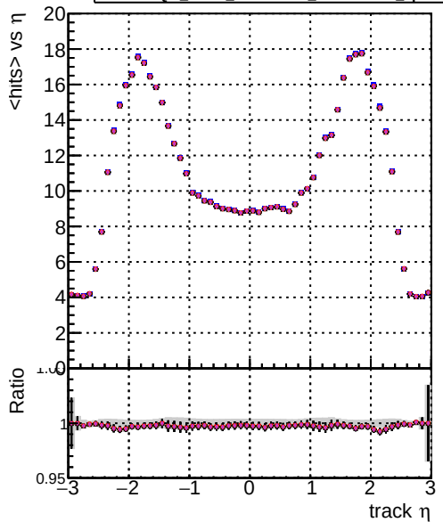
Legend for mean hits vs \eta : DOM mkFit XiMinusPU tetaInLowpt specPless1-lowpt DOM mkFit XiMinusPU NEWdefault specPless2-lowpt DOM mkFit XiMinusPU NEWdefault specPless3-lowpt DOM mkFit XiMinusPU NEWdefault specPless4-lowpt
