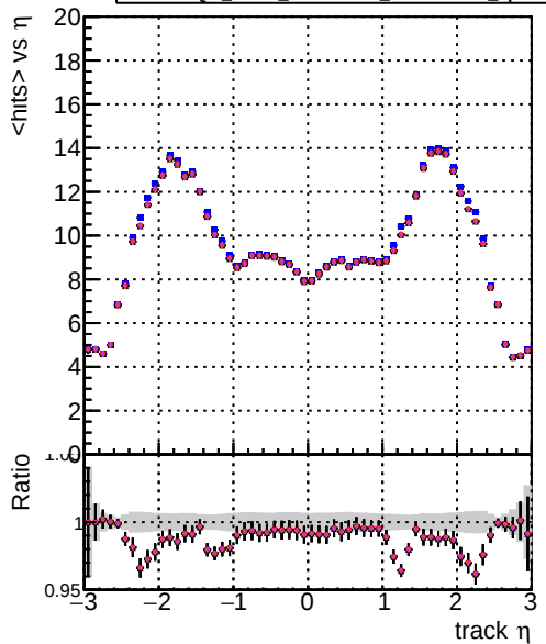
Legend for mean hits vs \eta : DOM mkFit XiMinusPU tetaair-lowpt DOM mkFit XiMinusPU NEWdefault specPless1-lowpt DOM mkFit XiMinusPU NEWdefault specPless2-lowpt DOM mkFit XiMinusPU NEWdefault specPless3-lowpt DOM mkFit XiMinusPU NEWdefault specPless4-lowpt
