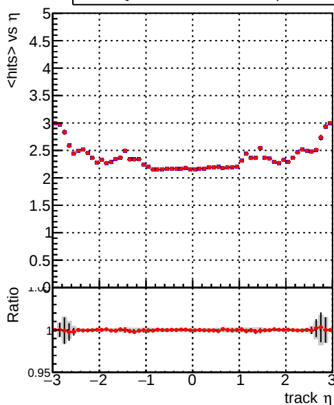
mean hits vs \eta Legend: DQM_mkFit_XiMinusPU_retrain2-lowpt (blue line), DQM_mkFit_XiMinusPUold-lowpt (red line)
