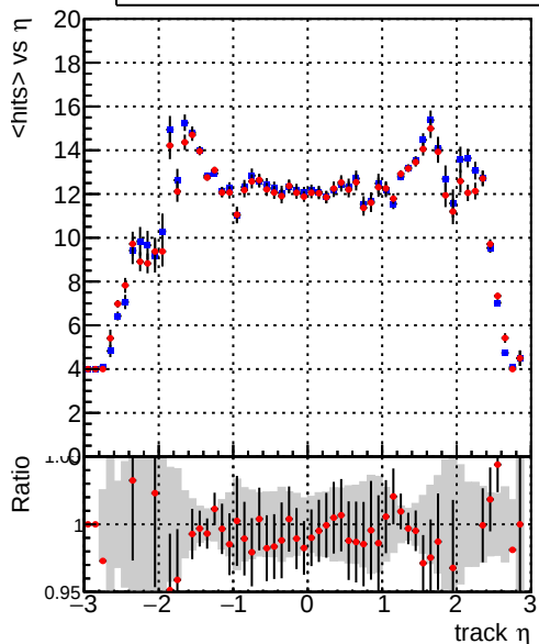
mean hits vs \eta Legend: \square DQM_mkFit_XiMinusPU_retrain2-lowpt (blue), \square DQM_mkFit_XiMinusPUold-lowpt (red)
