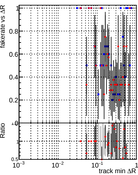
Legend: DQM_mkFit_XiMinusPU_retrain2-lowpt (blue squares), DQM_mkFit_XiMinusPUold-lowpt (red circles)
