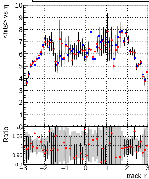
mean hits vs \eta Legend: DQM_mkFit_XiMinusPU_retrain2-lowpt (blue line with error bars), DQM_mkFit_XiMinusPUold-lowpt (red line with error bars)
