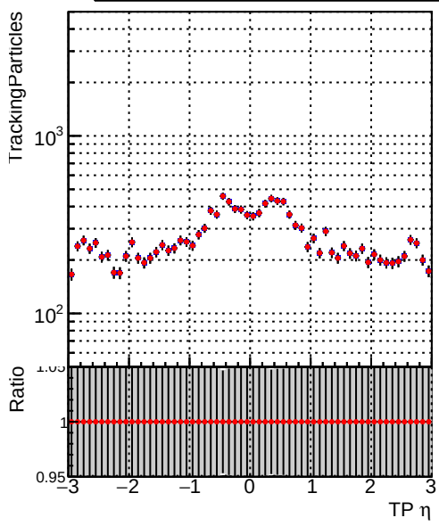
Legend: - DQM_mkFit_XiMinusPU_retrain2-lowpt (blue diamonds) - DQM_mkFit_XiMinusPUold-lowpt (red diamonds)
