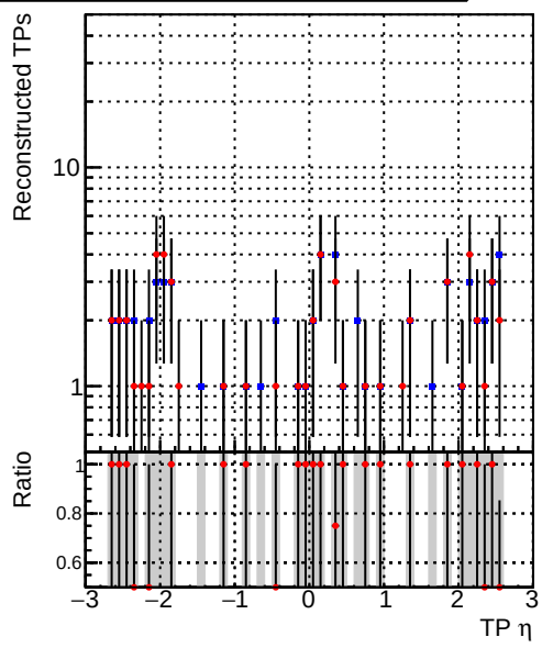
Legend: - DQM_mkFit_XiMinusPU_retrain2-lowpt (blue diamonds) - DQM_mkFit_XiMinusPUold-lowpt (red diamonds)
