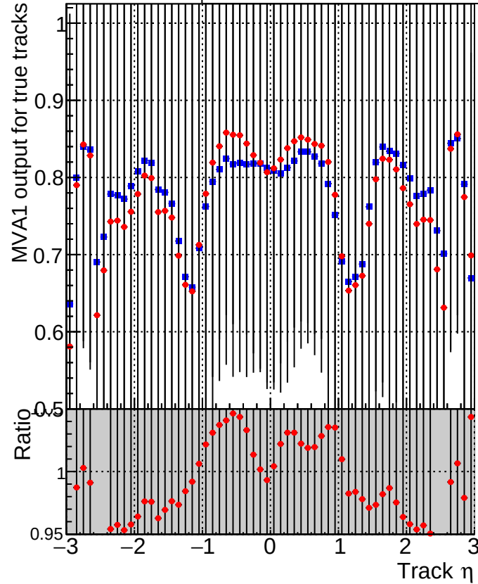
MVA1 of associated tracks (recoToSim) vs. track \eta ■ DQM_mkFit_XiMinusPU_retrain2-lowpt ● DQM_mkFit_XiMinusPUold-lowpt
