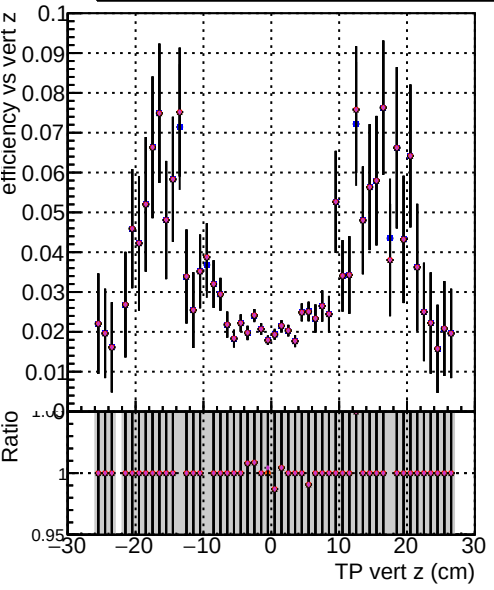
Efficiency vs vertpos DOM mkFit XiMinusPU retranz2-lowpt DOM mkFit XiMinusPU NEWdefault specPLess1-2-lowpt DOM mkFit XiMinusPU NEWdefault specPLess2-2-lowpt DOM mkFit XiMinusPU NEWdefault specPLess3-2-lowpt DOM mkFit XiMinusPU NEWdefault specPLess4-2-lowpt
