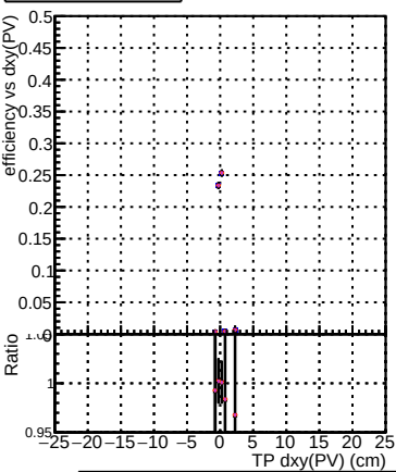
Efficiency vs Dxy(PV) DOM_mkFit_XiMinusPU_retrain2-lowpt DOM_mkFit_XiMinusPU_NEWdefault_specPLess1-2-lowpt DOM_mkFit_XiMinusPU_NEWdefault_specPLess2-2-lowpt DOM_mkFit_XiMinusPU_NEWdefault_specPLess3-2-lowpt DOM_mkFit_XiMinusPU_NEWdefault_specPLess4-2-lowpt
