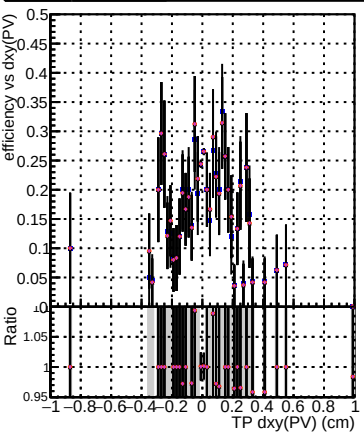
Efficiency vs Dxy(PV) DOM_mkFit_XiMinusPU_retrain2-lowpt DOM_mkFit_XiMinusPU_NEWdefault_specPLess1-2-lowpt DOM_mkFit_XiMinusPU_NEWdefault_specPLess2-2-lowpt DOM_mkFit_XiMinusPU_NEWdefault_specPLess3-2-lowpt DOM_mkFit_XiMinusPU_NEWdefault_specPLess4-2-lowpt
