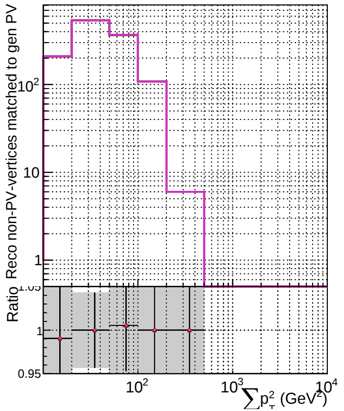
RecoAssoc2GenPVMatchedNotHighest_Pt2
