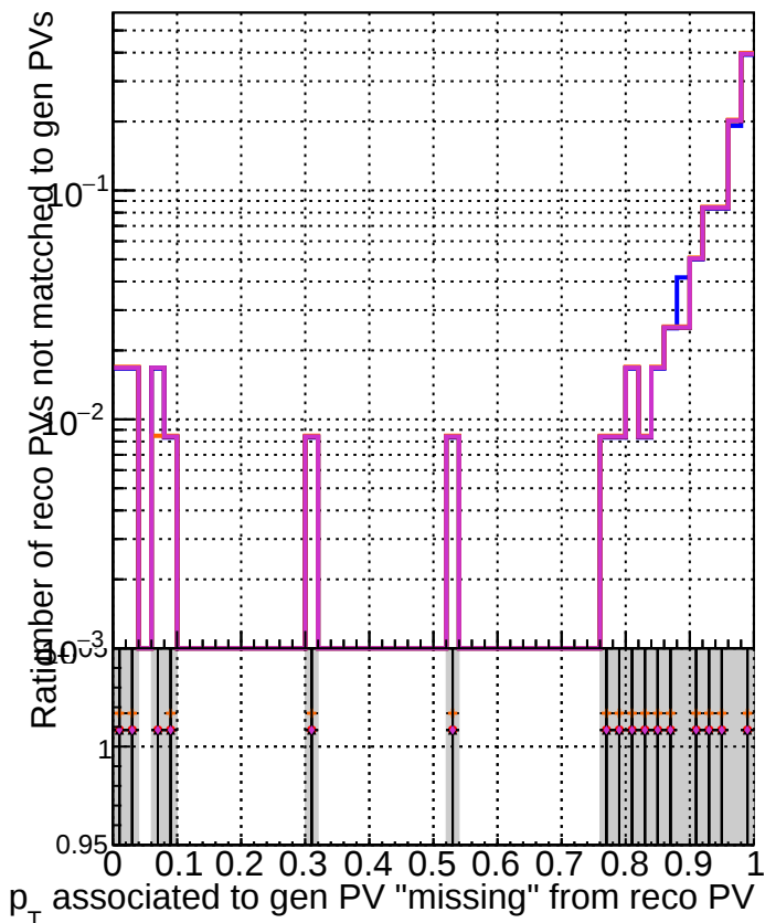
specPless4-z-lowpl RECOPVASSOCZGENPVINOTMATCHED_MISSING
